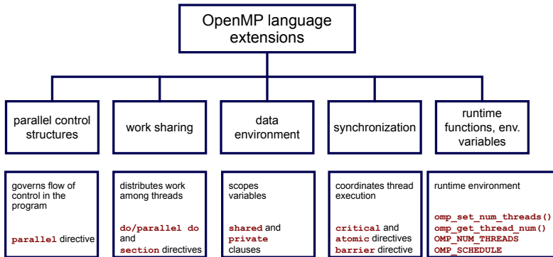
Figure: Classification of the OpenMP extensions by tasks of the elements 4 .
